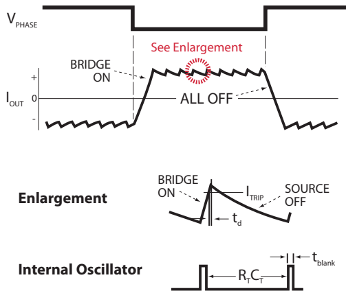
Figure 3: Thermal Protection
