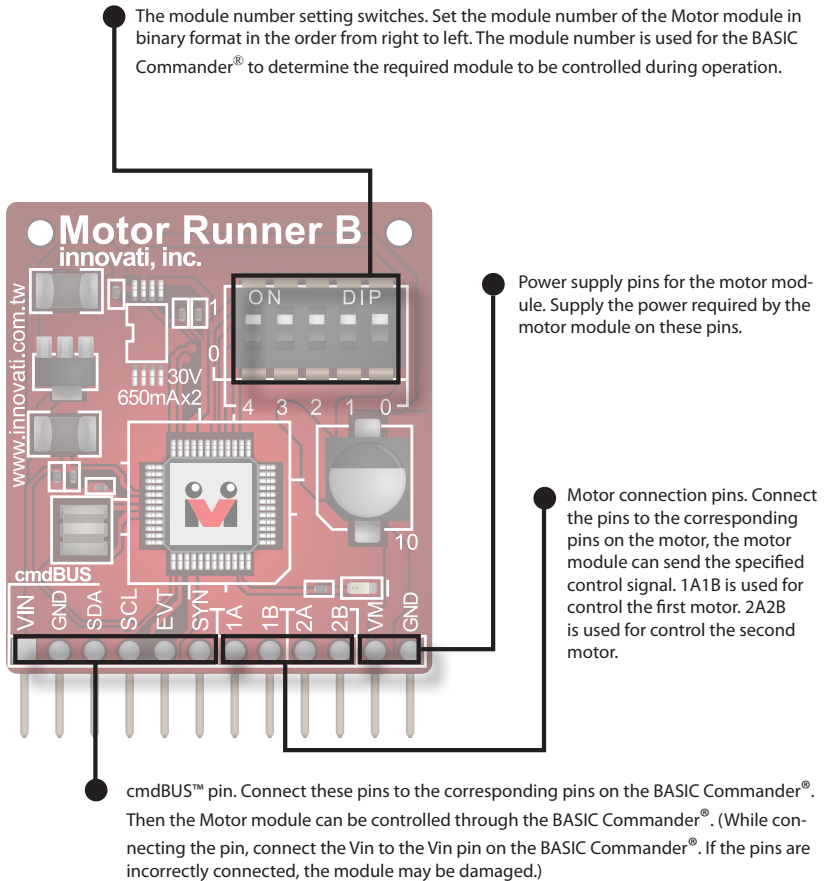
Figure 2: Module And Switch Pin Assignment
